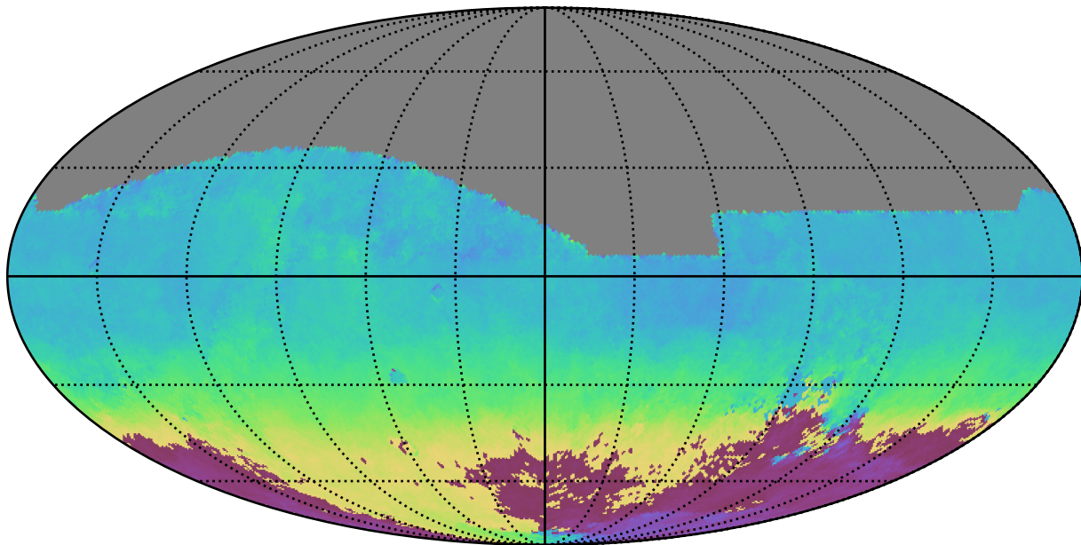
baseline_v3.2_10yrs All sky z band: AngleMean rotSkyPos
