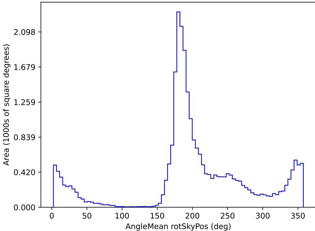
baseline_v3.2_10yrs All sky z band: AngleMean rotSkyPos
