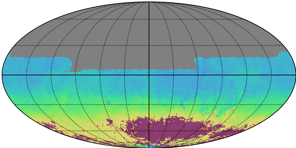
baseline_v3.2_10yrs All sky y band: AngleMean rotSkyPos
