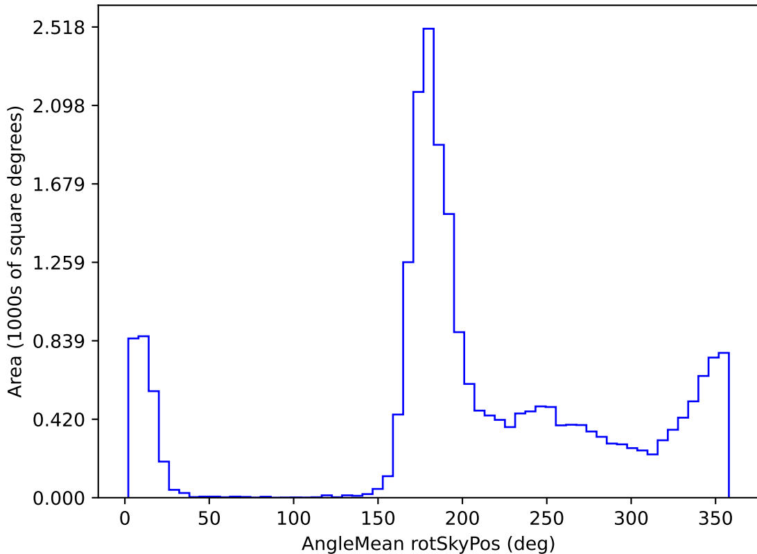
baseline_v3.2_10yrs All sky y band: AngleMean rotSkyPos
