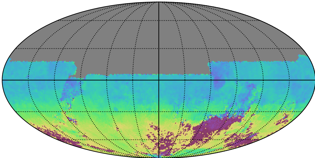
baseline_v3.2_10yrs All sky u band: AngleMean rotSkyPos
