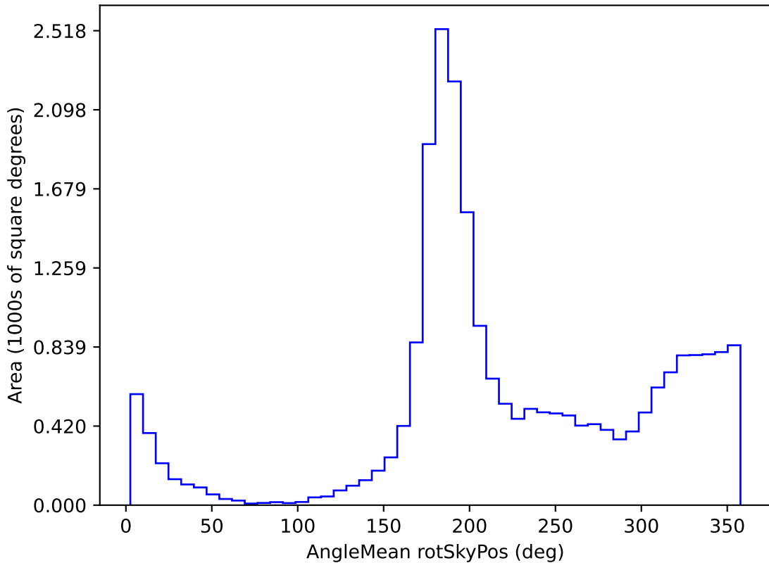
baseline_v3.2_10yrs All sky u band: AngleMean rotSkyPos
