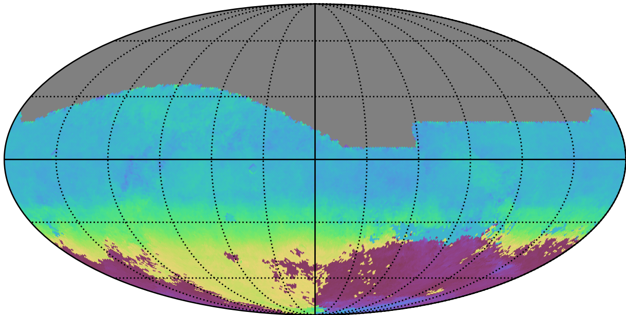
baseline_v3.2_10yrs All sky r band: AngleMean rotSkyPos
