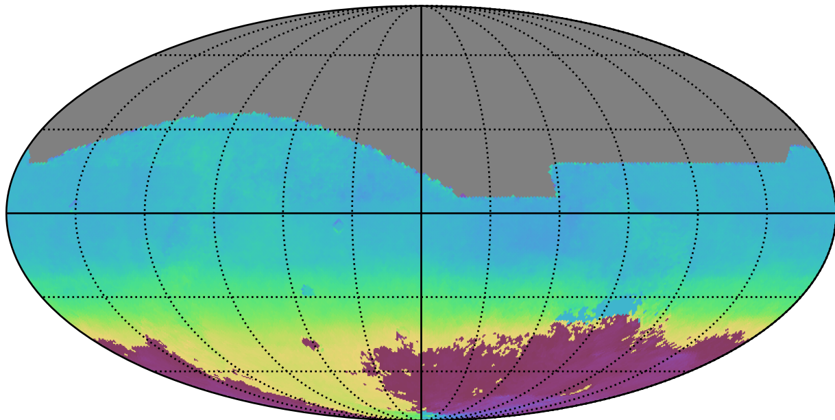
baseline_v3.2_10yrs All sky all bands: AngleMean rotSkyPos
