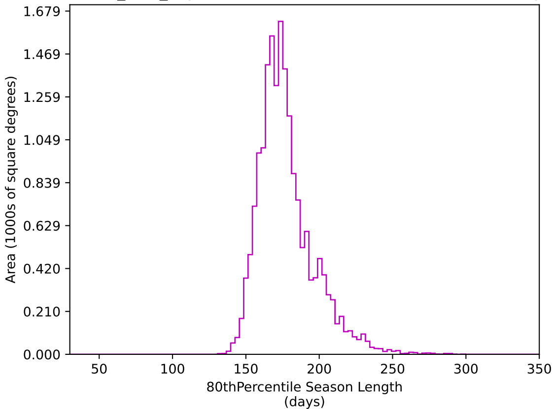
baseline_v3.2_10yrs WFD z band: 80thPercentile Season Length
