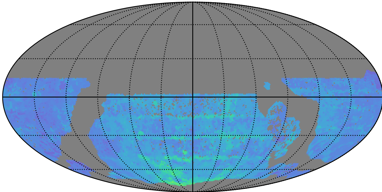
baseline_v3.2_10yrs WFD y band: 80thPercentile Season Length
