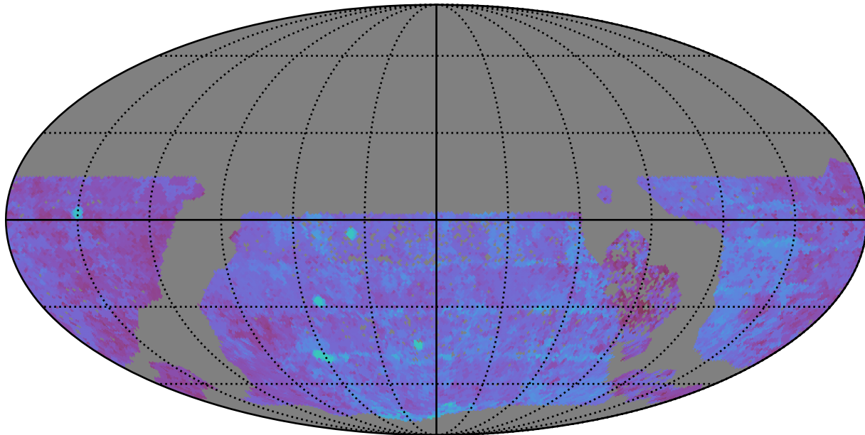
baseline_v3.2_10yrs WFD u band: 80thPercentile Season Length
