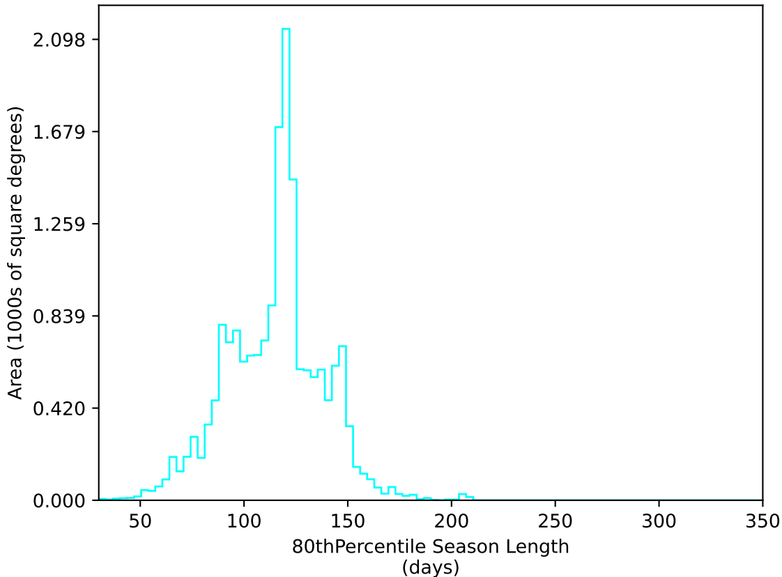
baseline_v3.2_10yrs WFD u band: 80thPercentile Season Length
