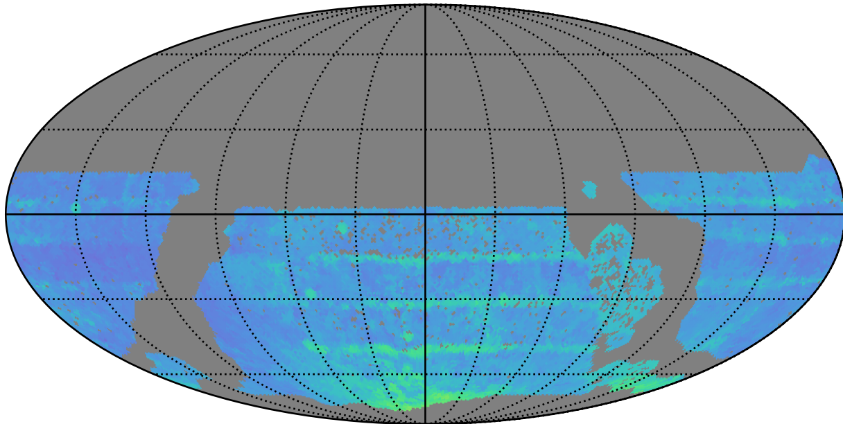
baseline_v3.2_10yrs WFD r band: 80thPercentile Season Length
