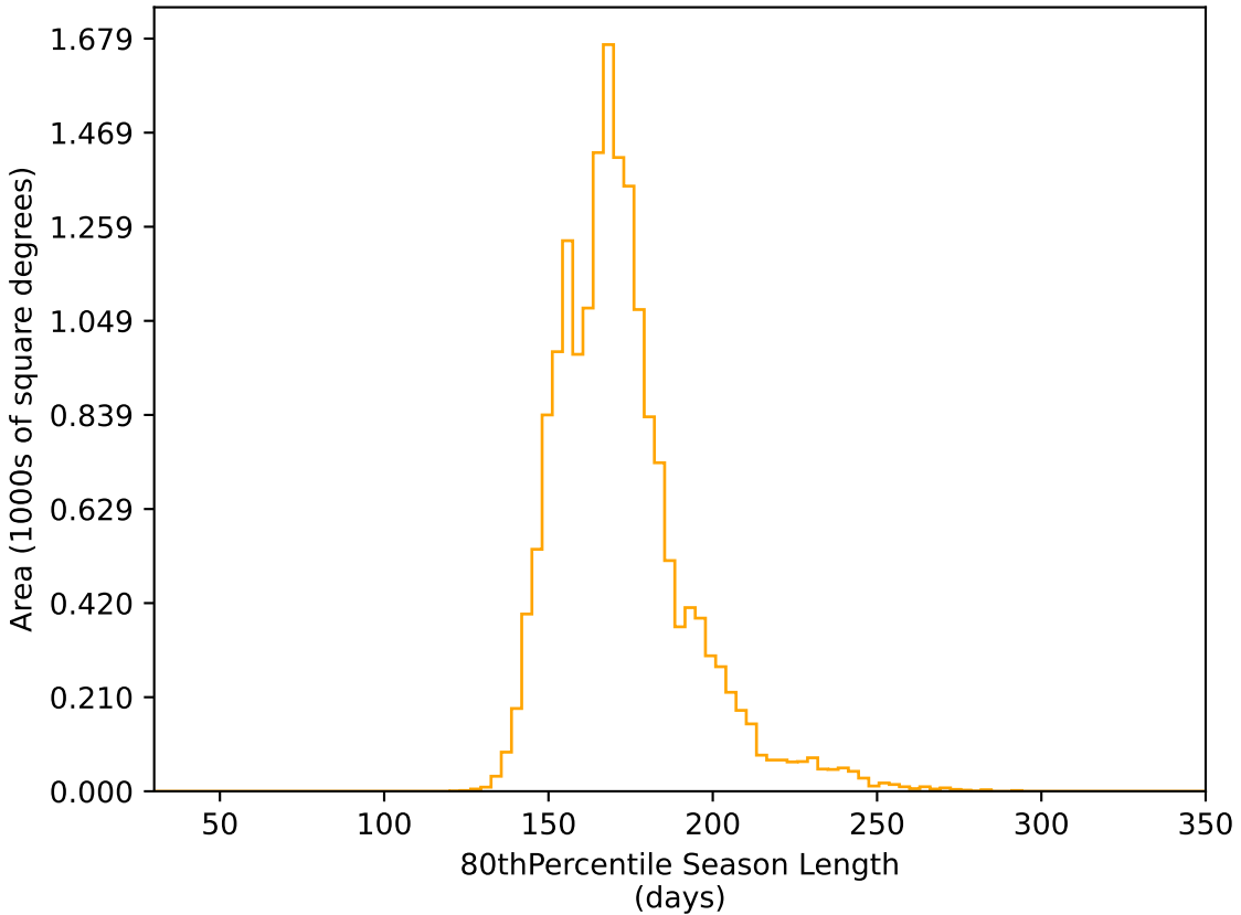
baseline_v3.2_10yrs WFD r band: 80thPercentile Season Length
