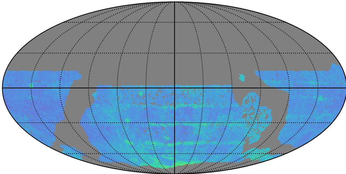
baseline_v3.2_10yrs WFD i band: 80thPercentile Season Length
