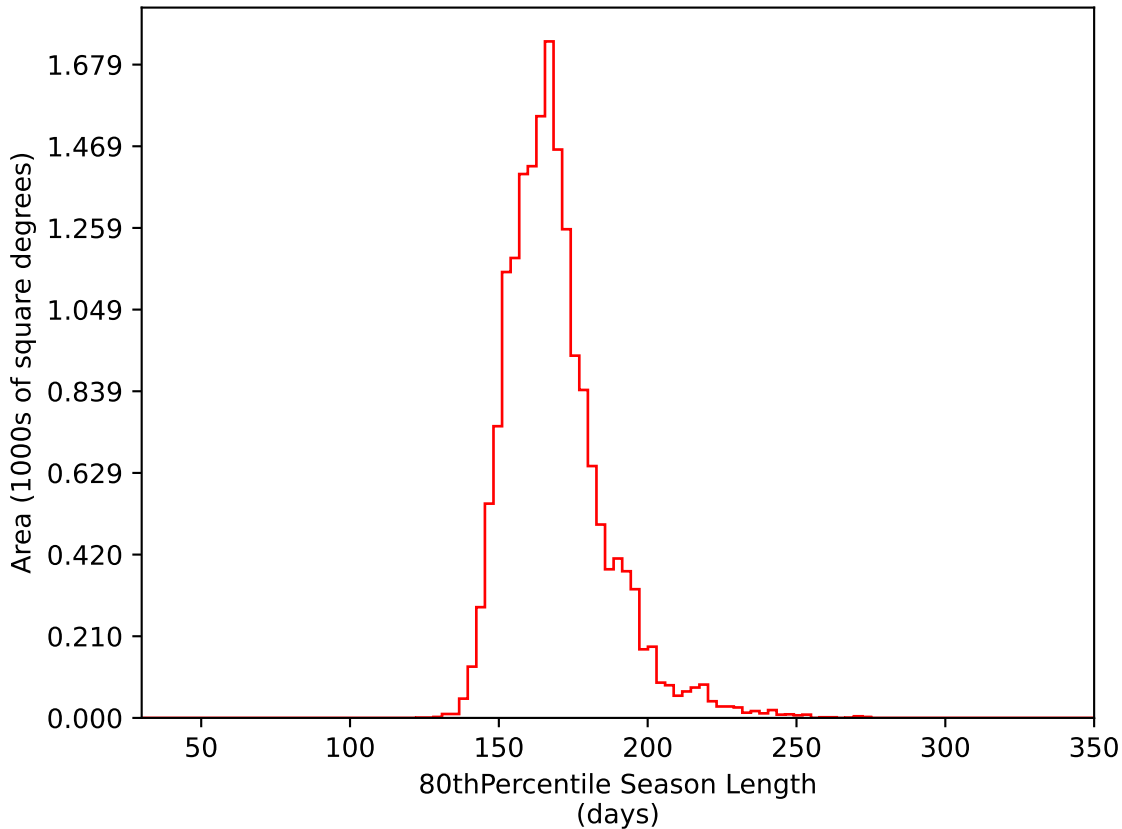
baseline_v3.2_10yrs WFD i band: 80thPercentile Season Length
