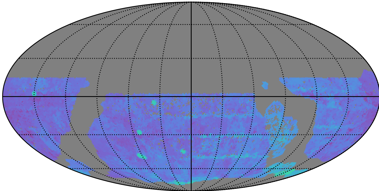
baseline_v3.2_10yrs WFD g band: 80thPercentile Season Length
