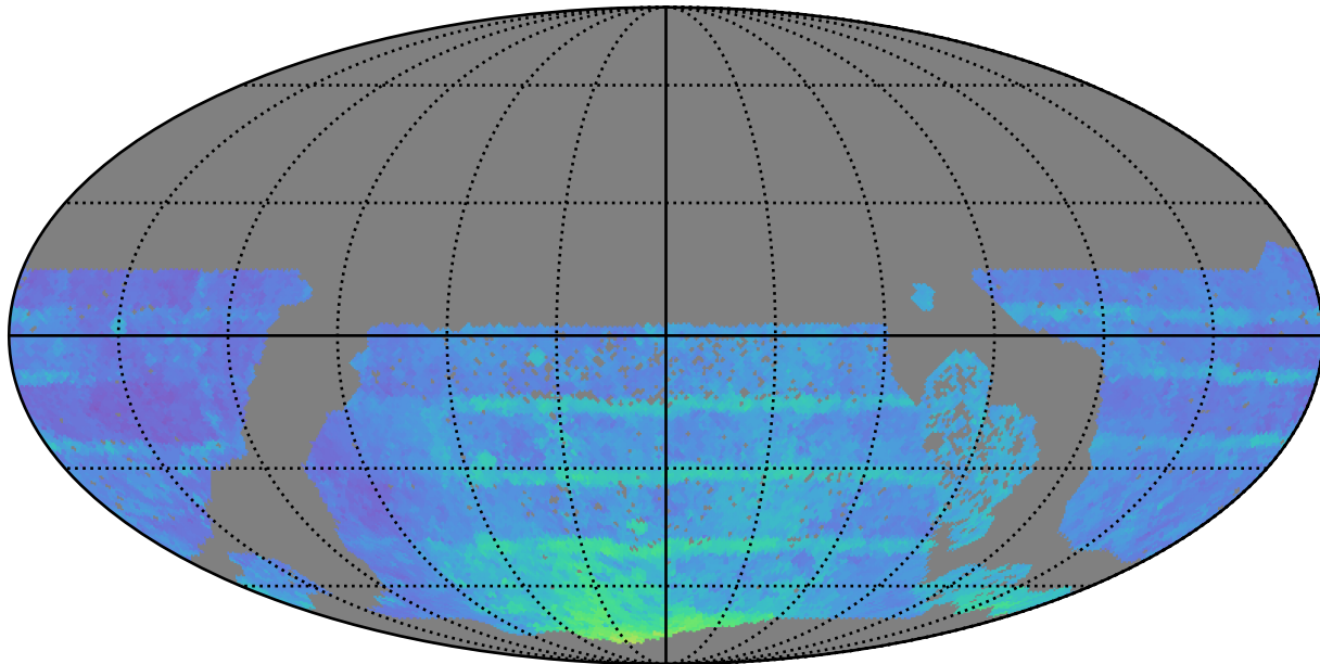
baseline_v3.2_10yrs WFD all bands: 80thPercentile Season Length
