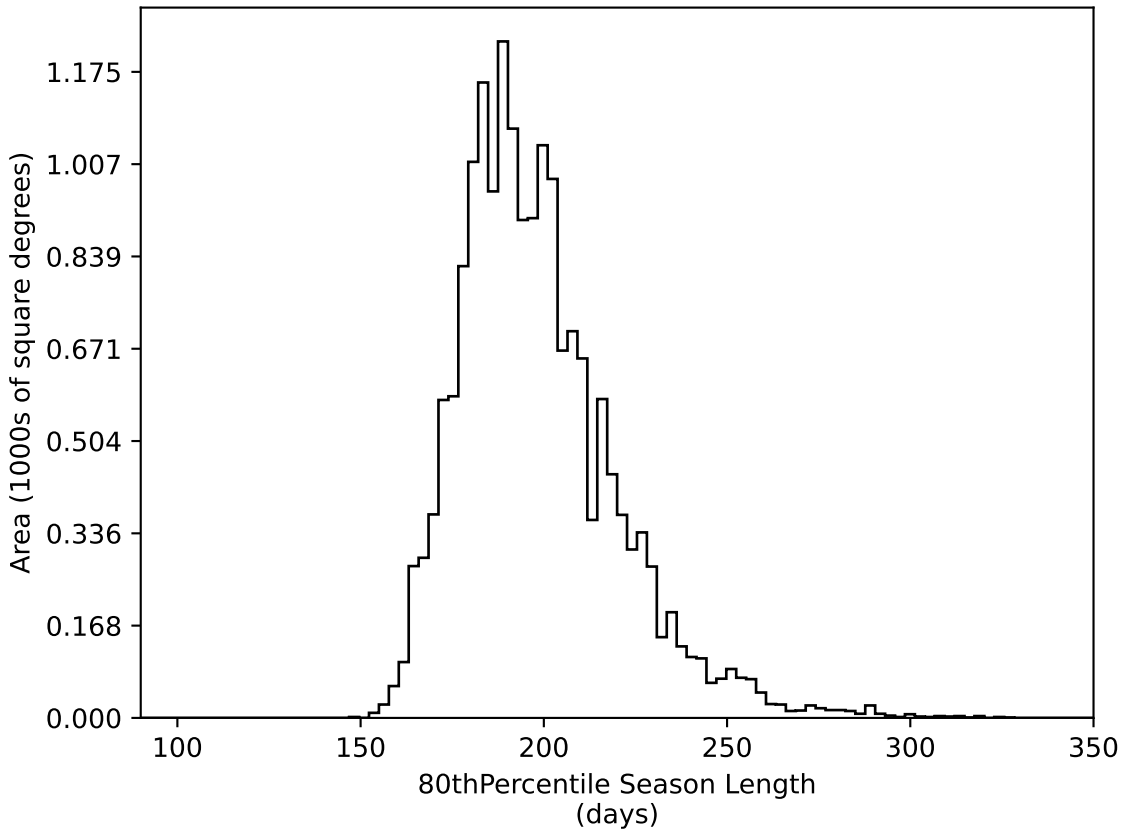
baseline_v3.2_10yrs WFD all bands: 80thPercentile Season Length
