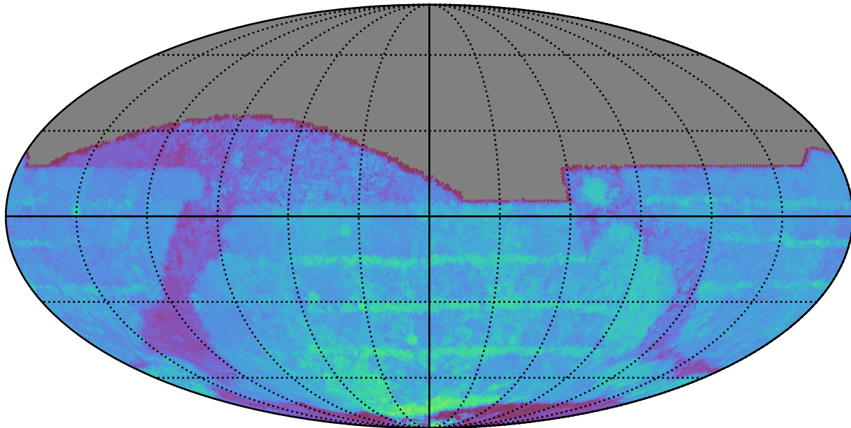
baseline_v3.2_10yrs All sky z band: 80thPercentile Season Length
