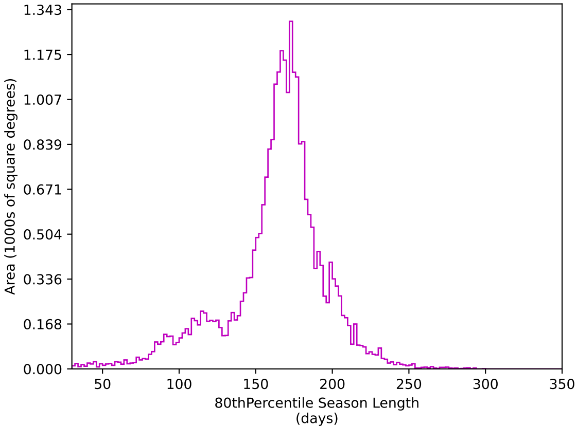
baseline_v3.2_10yrs All sky z band: 80thPercentile Season Length
