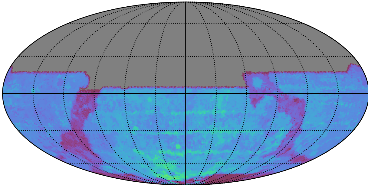
baseline_v3.2_10yrs All sky y band: 80thPercentile Season Length
