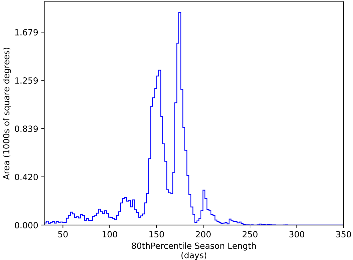
baseline_v3.2_10yrs All sky y band: 80thPercentile Season Length
