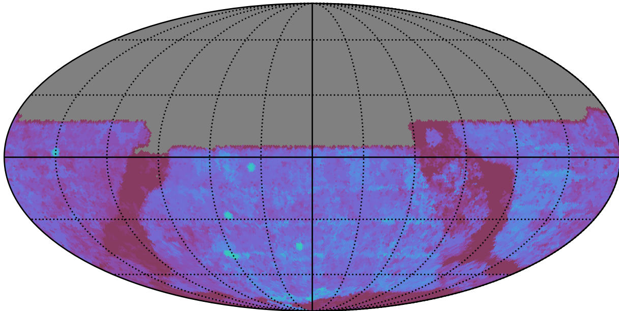
baseline_v3.2_10yrs All sky u band: 80thPercentile Season Length
