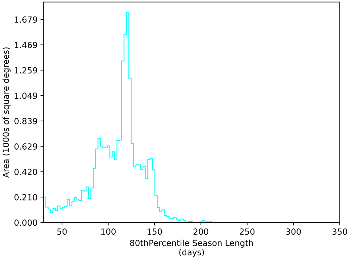
baseline_v3.2_10yrs All sky u band: 80thPercentile Season Length
