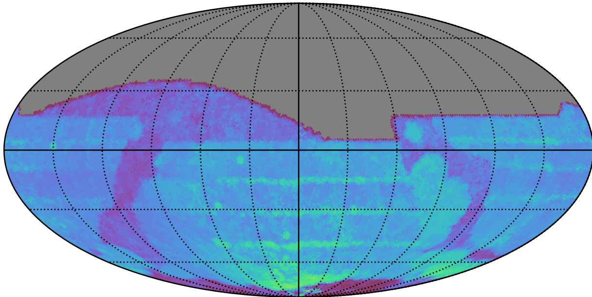
baseline_v3.2_10yrs All sky r band: 80thPercentile Season Length
