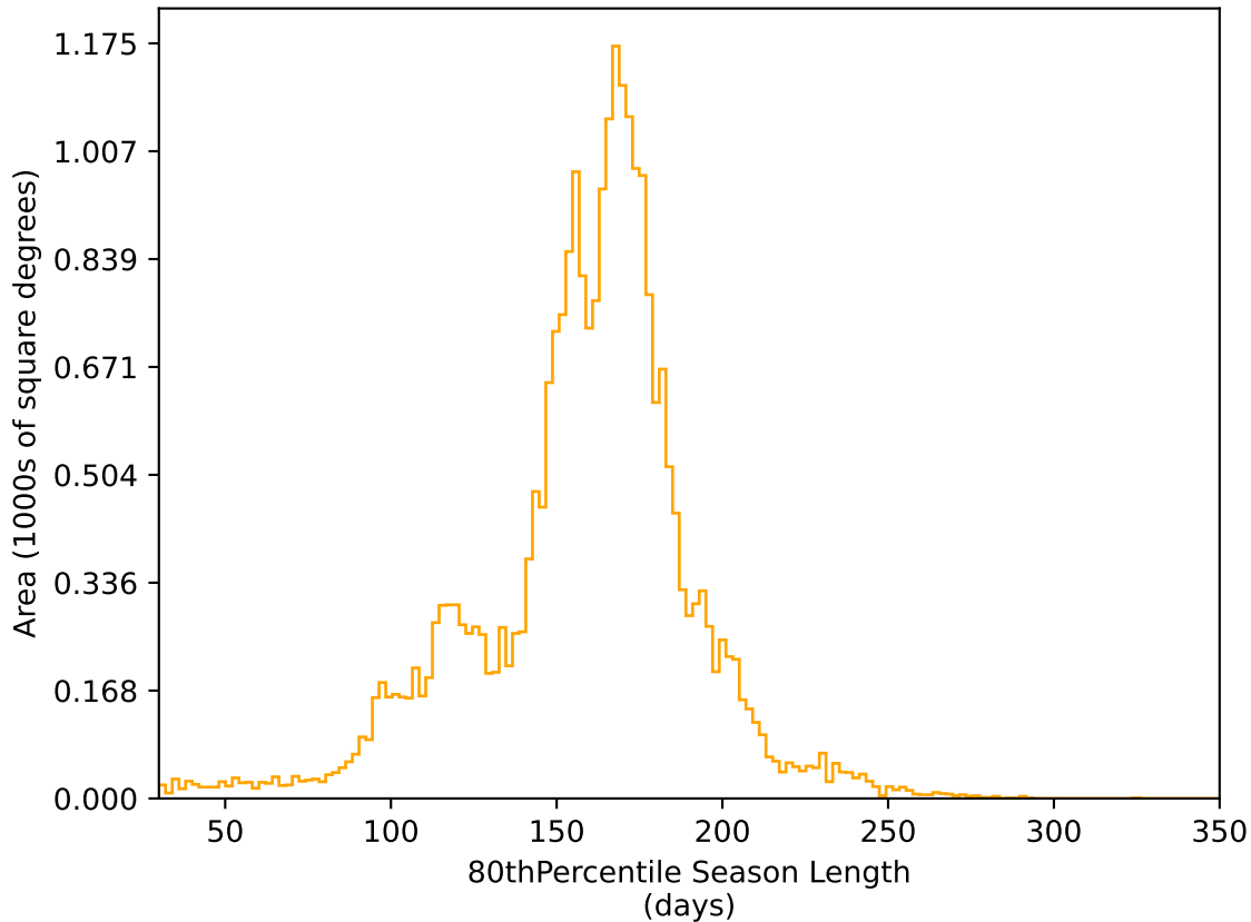
baseline_v3.2_10yrs All sky r band: 80thPercentile Season Length
