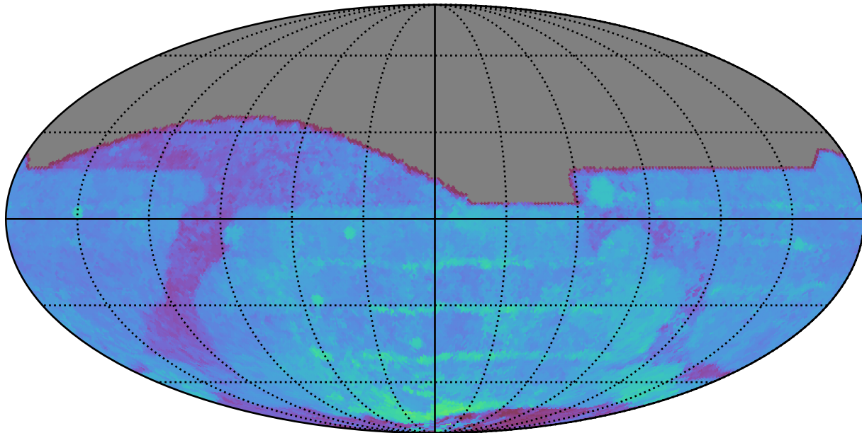
baseline_v3.2_10yrs All sky i band: 80thPercentile Season Length
