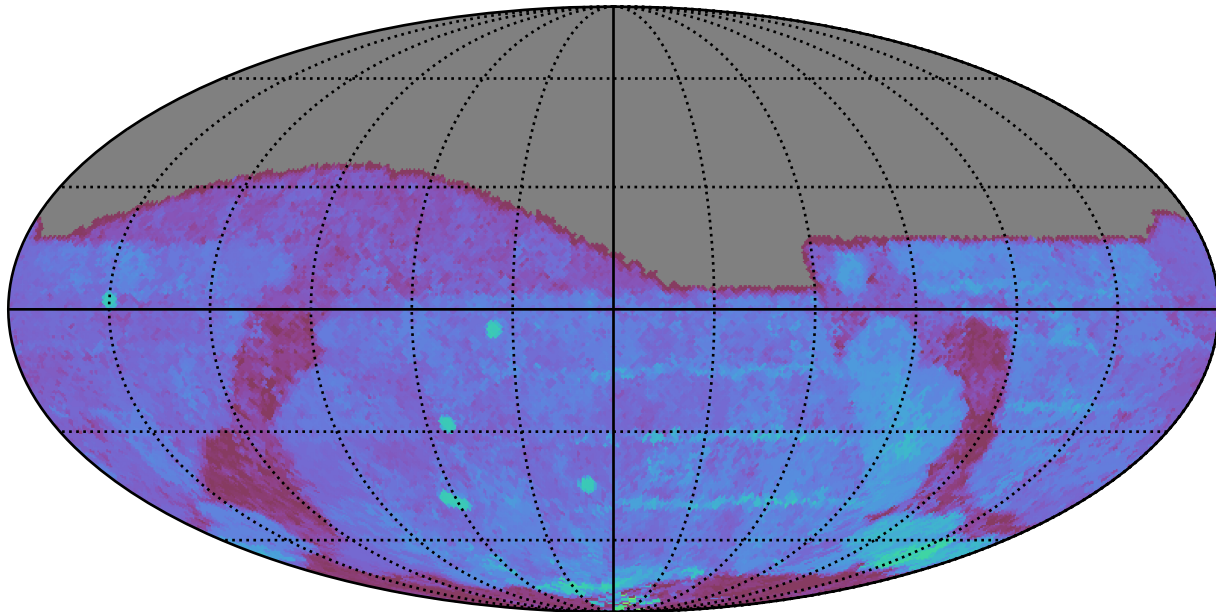
baseline_v3.2_10yrs All sky g band: 80thPercentile Season Length
