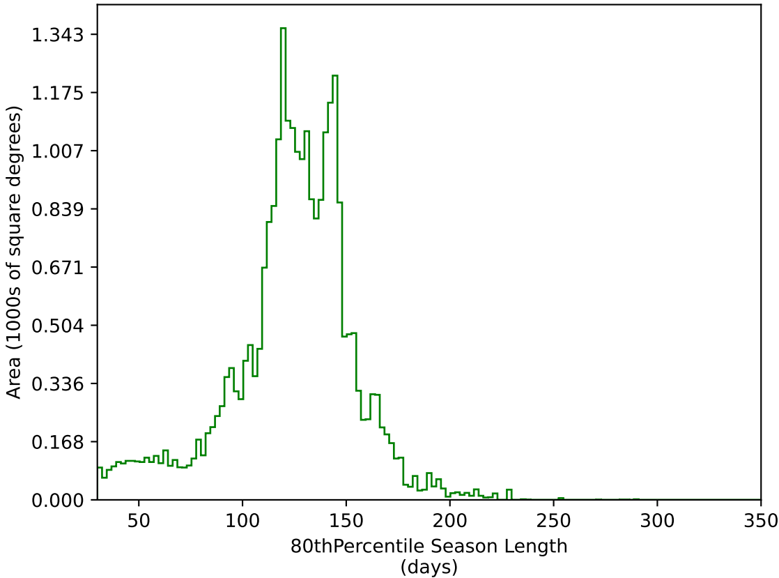
baseline_v3.2_10yrs All sky g band: 80thPercentile Season Length
