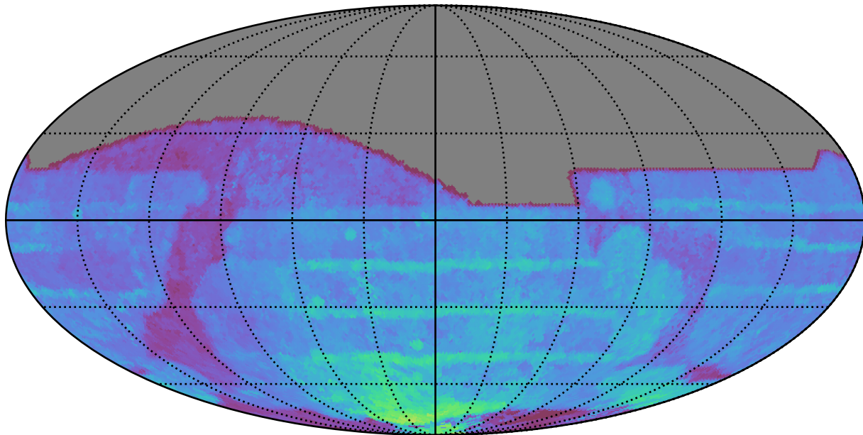
baseline_v3.2_10yrs All sky all bands: 80thPercentile Season Length
