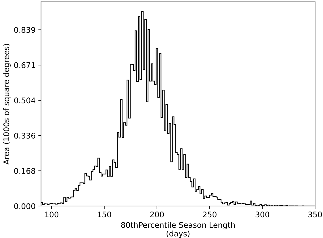
baseline_v3.2_10yrs All sky all bands: 80thPercentile Season Length
