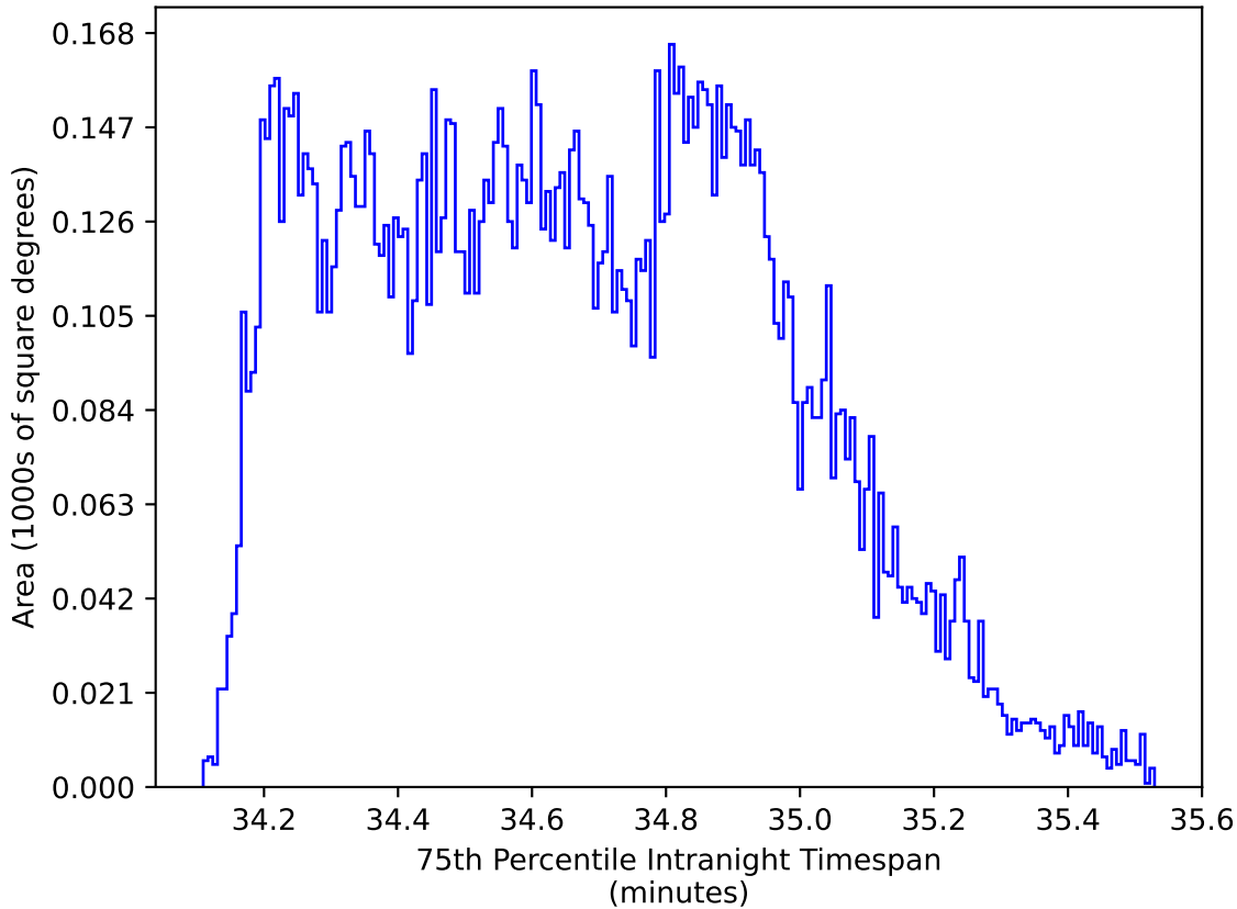
baseline_v3.2_10yrs WFD zy bands: 75th Percentile Intranight Timespan
