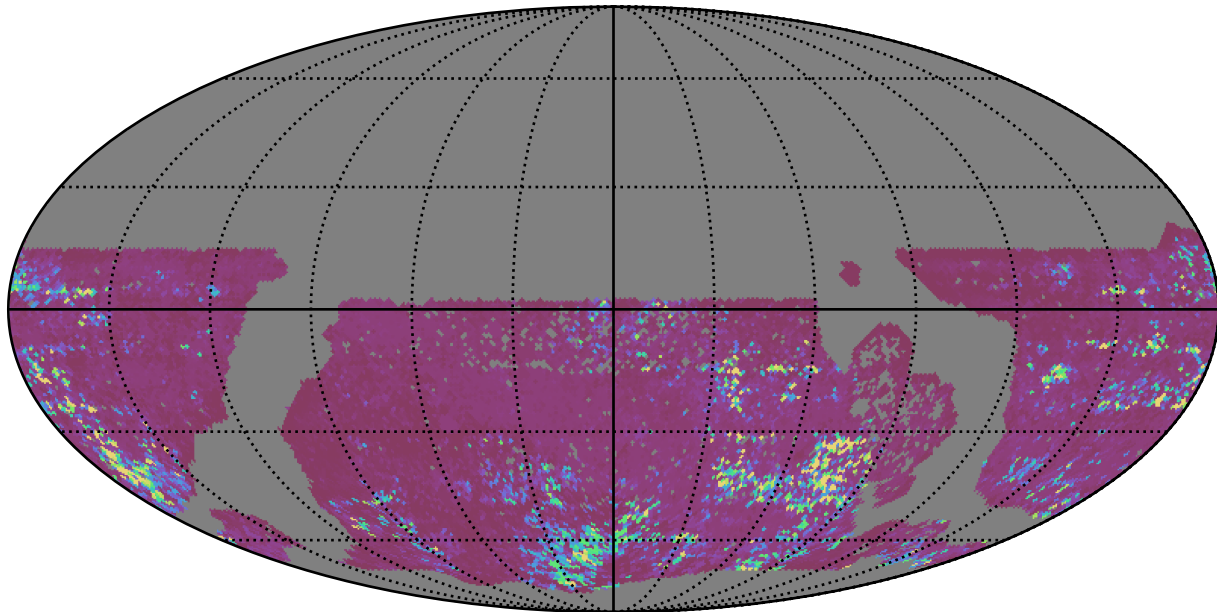
baseline_v3.2_10yrs WFD z band: 75th Percentile Intranight Timespan
