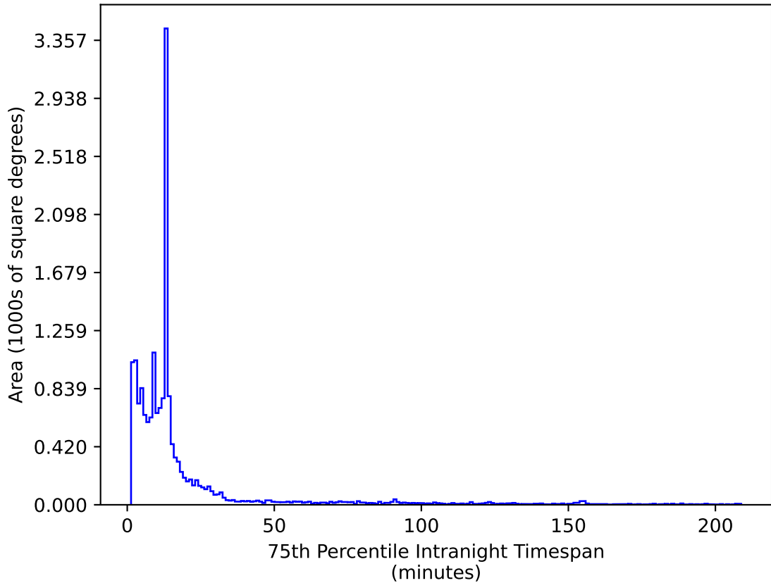
baseline_v3.2_10yrs WFD z band: 75th Percentile Intranight Timespan
