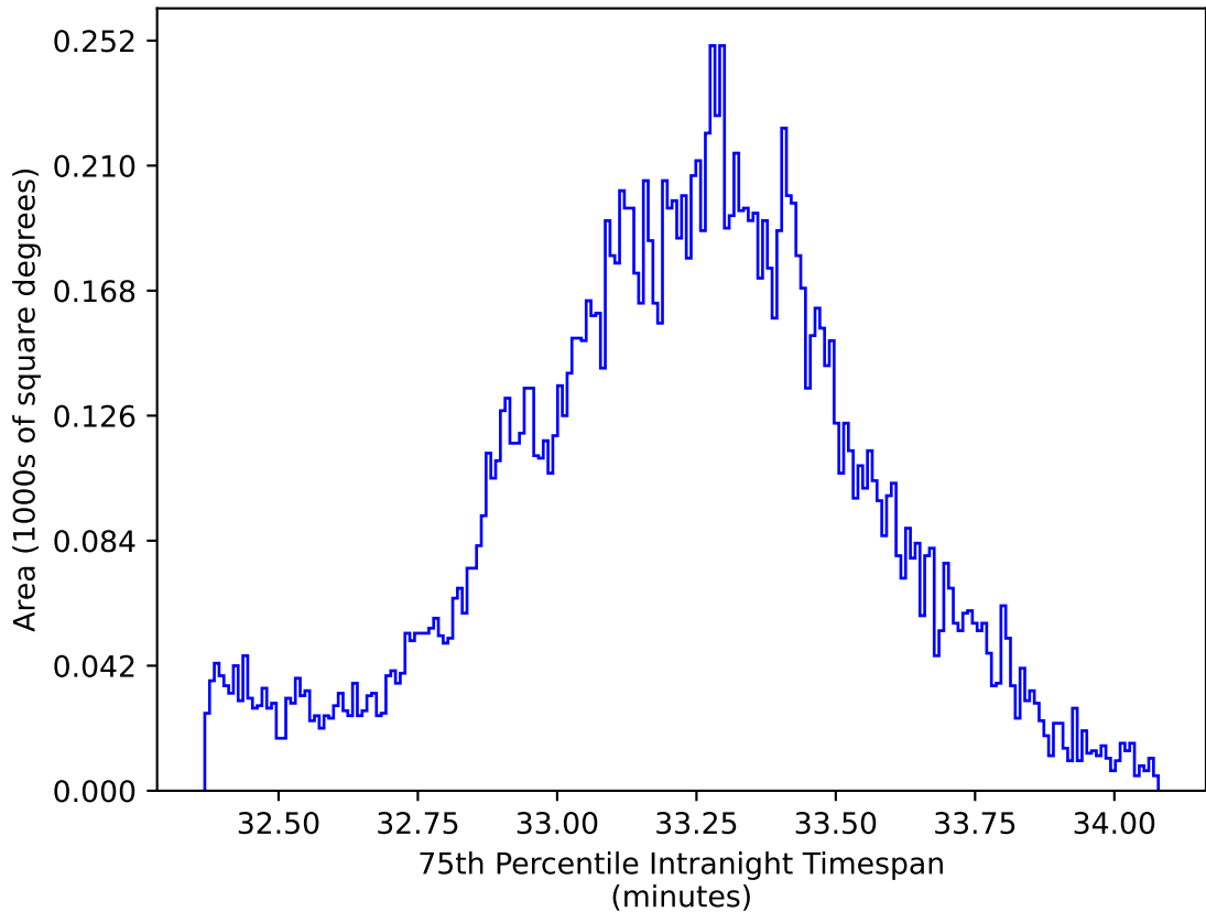
baseline_v3.2_10yrs WFD y band: 75th Percentile Intranight Timespan
