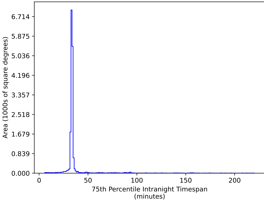
baseline_v3.2_10yrs WFD ug bands: 75th Percentile Intranight Timespan
