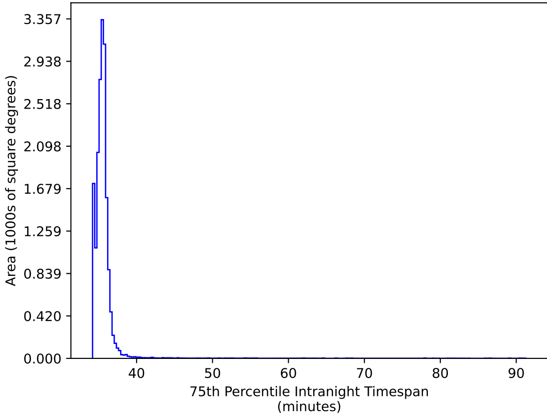
baseline_v3.2_10yrs WFD ri bands: 75th Percentile Intranight Timespan
