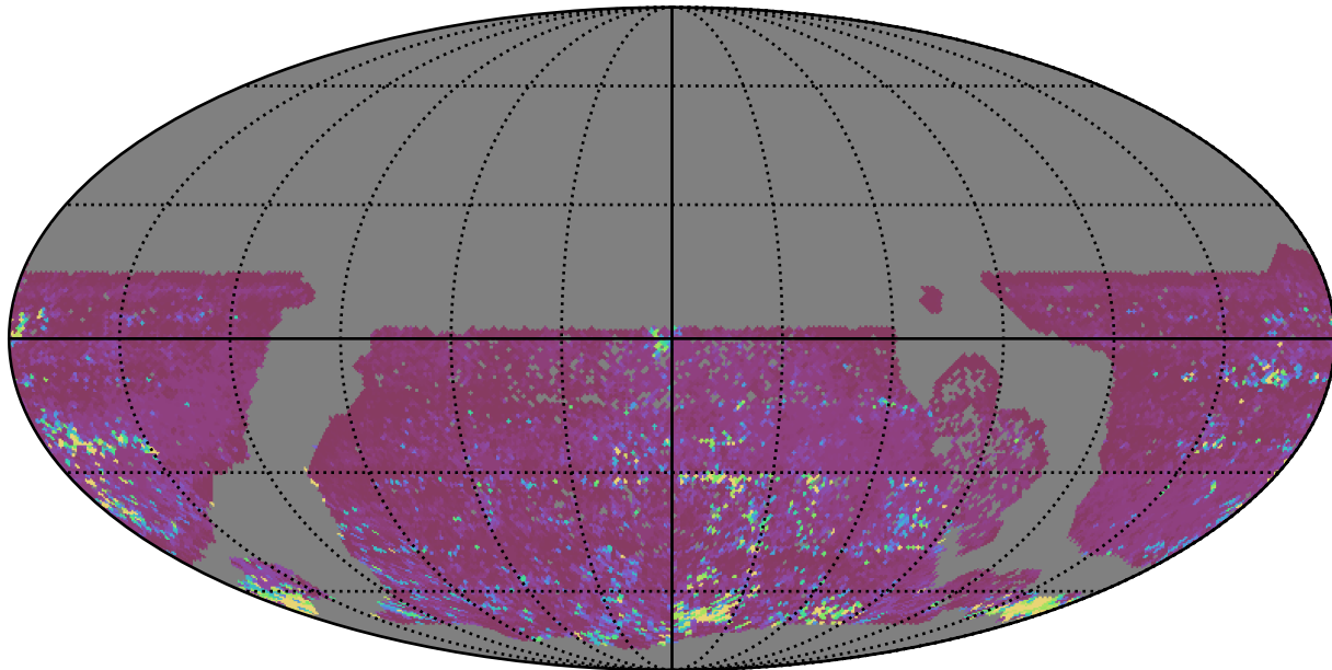
baseline_v3.2_10yrs WFD r band: 75th Percentile Intranight Timespan
