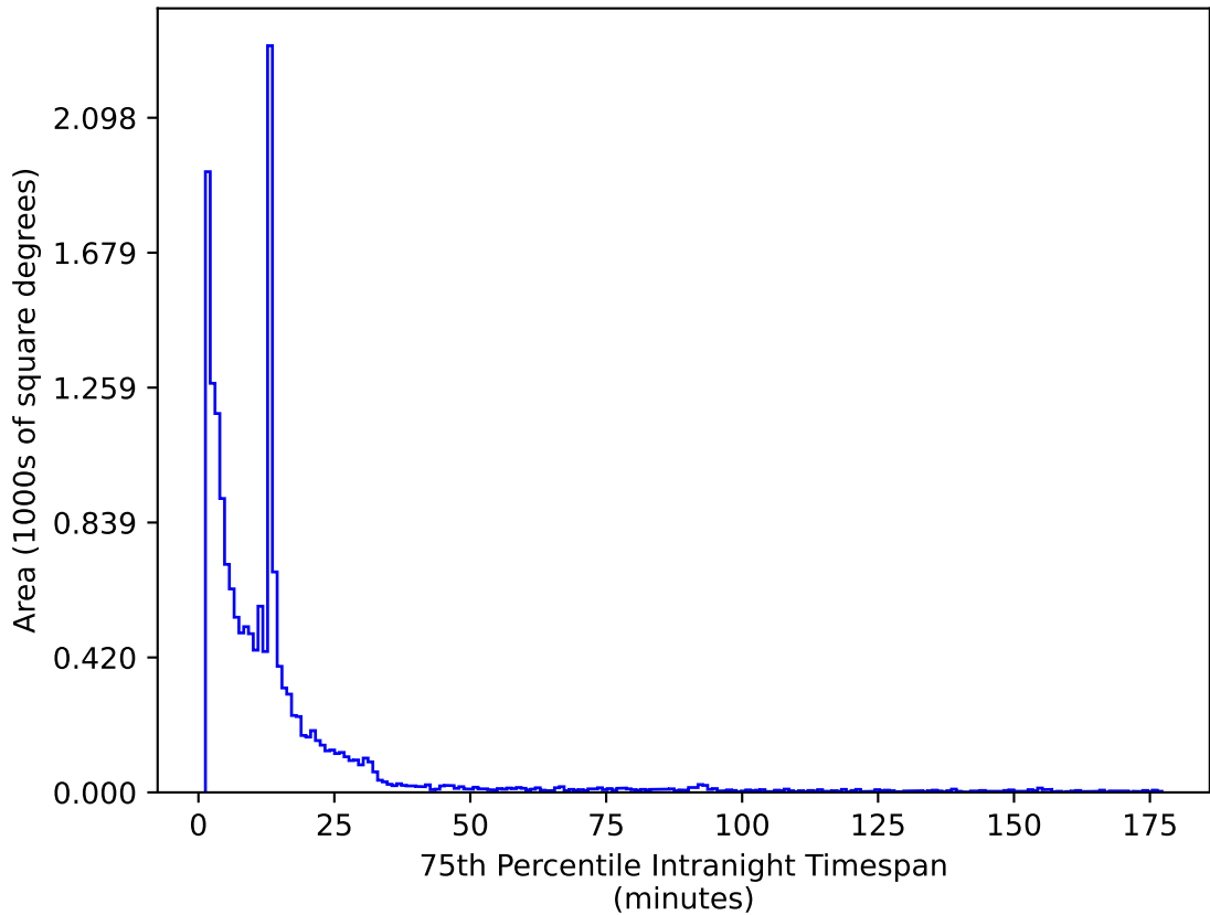
baseline_v3.2_10yrs WFD r band: 75th Percentile Intranight Timespan
