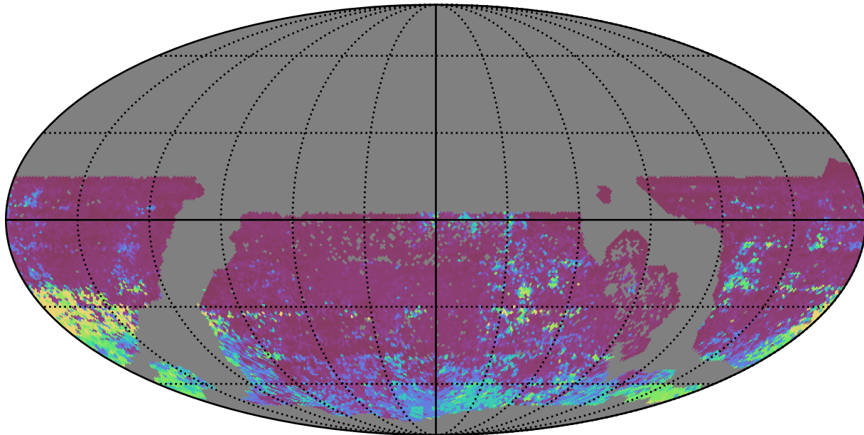
baseline_v3.2_10yrs WFD i band: 75th Percentile Intranight Timespan
