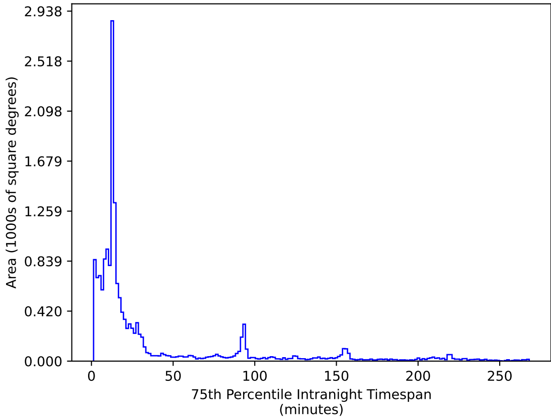
baseline_v3.2_10yrs WFD i band: 75th Percentile Intranight Timespan
