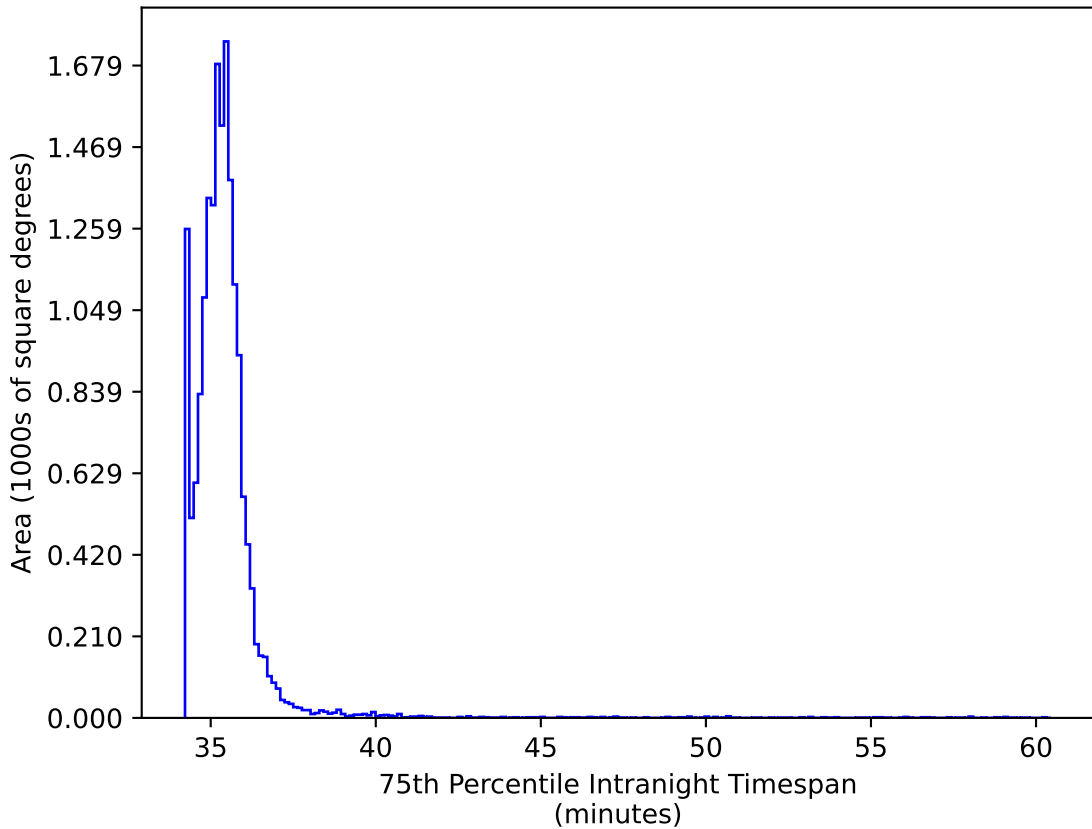
baseline_v3.2_10yrs WFD gr bands: 75th Percentile Intranight Timespan
