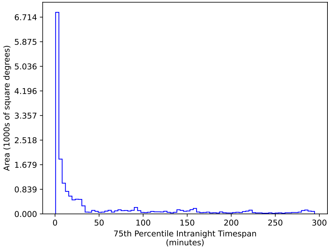
baseline_v3.2_10yrs WFD g band: 75th Percentile Intranight Timespan
