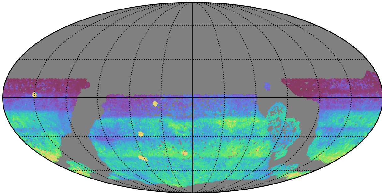
baseline_v3.2_10yrs WFD: 75th Percentile Intranight Timespan
