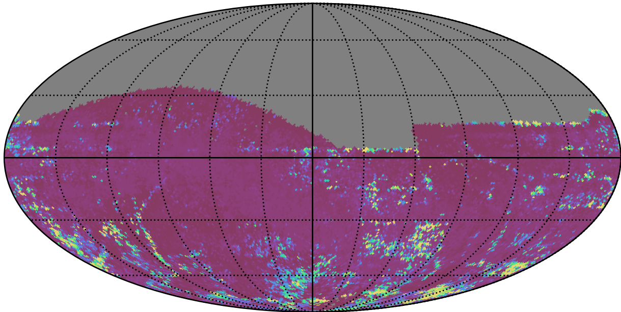
baseline_v3.2_10yrs All sky z band: 75th Percentile Intranight Timespan
