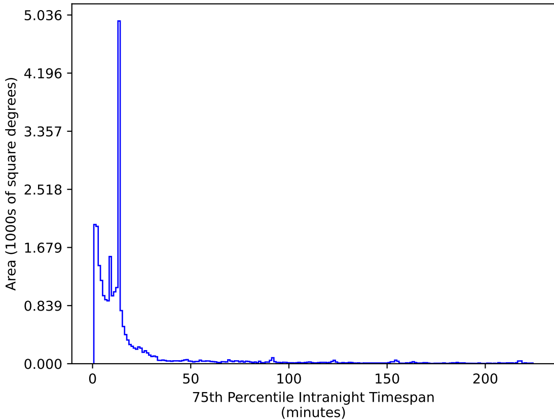
baseline_v3.2_10yrs All sky z band: 75th Percentile Intranight Timespan
