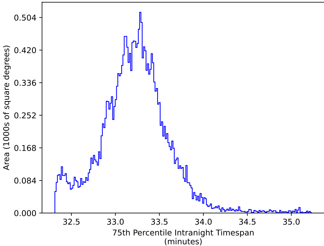
baseline_v3.2_10yrs All sky y band: 75th Percentile Intranight Timespan
