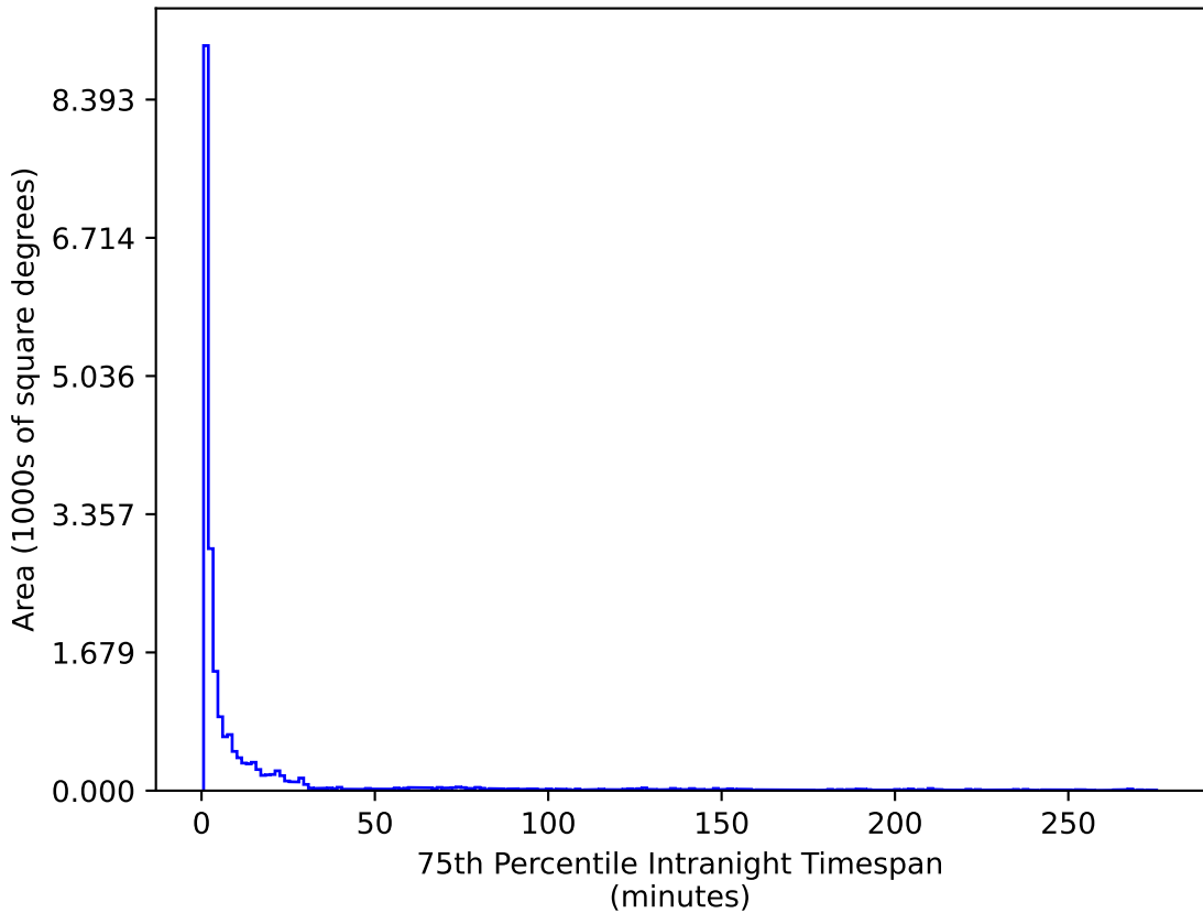
baseline_v3.2_10yrs All sky u band: 75th Percentile Intranight Timespan
