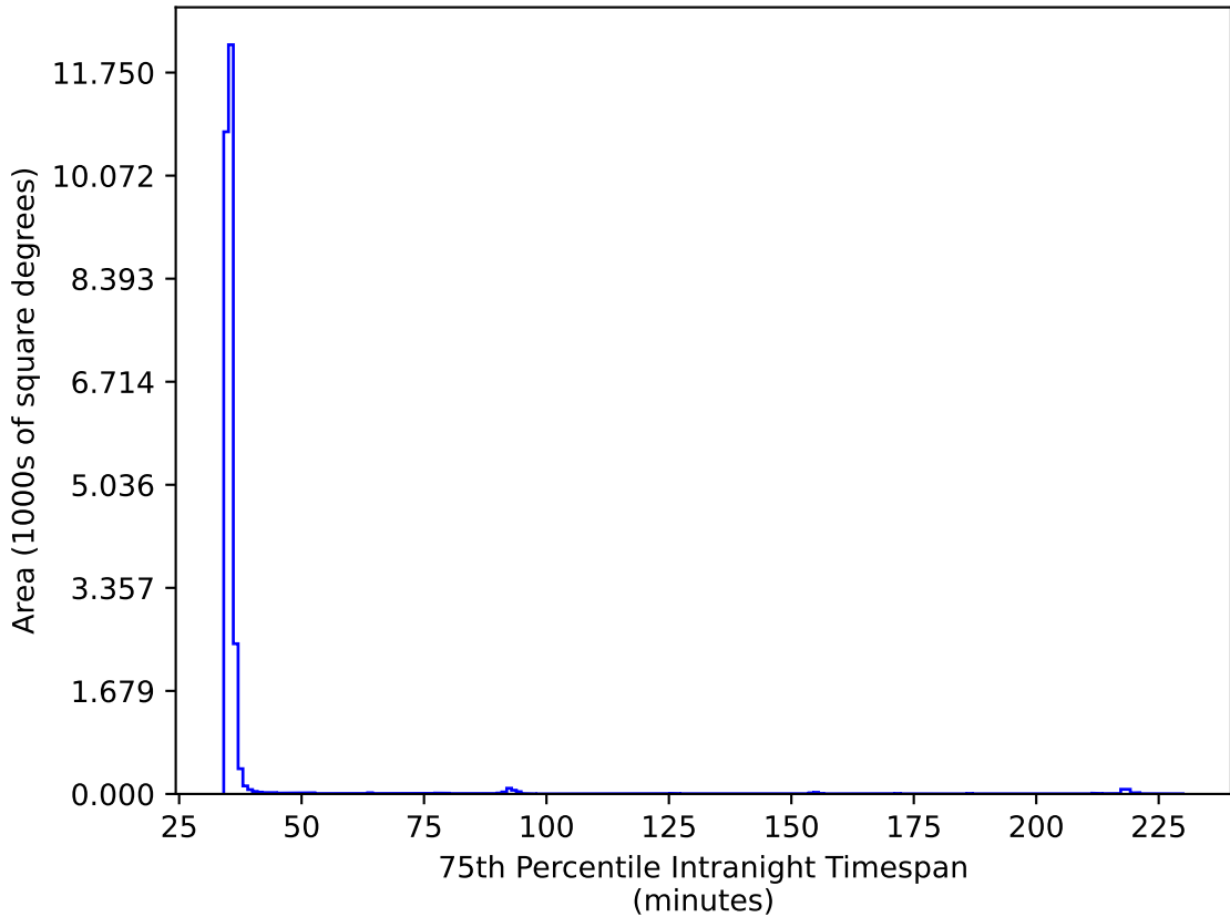
baseline_v3.2_10yrs All sky ri bands: 75th Percentile Intranight Timespan
